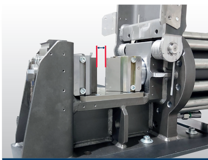
Adjustable blade spacing
