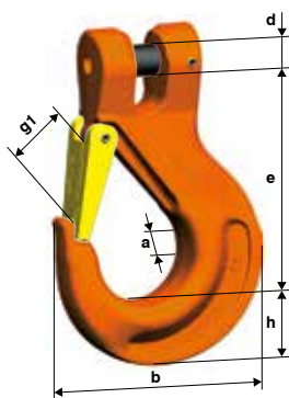
KHSW Kuppelhaken
